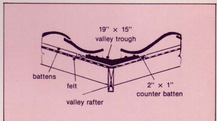
TYPICAL DETAIL OF VALLEY
