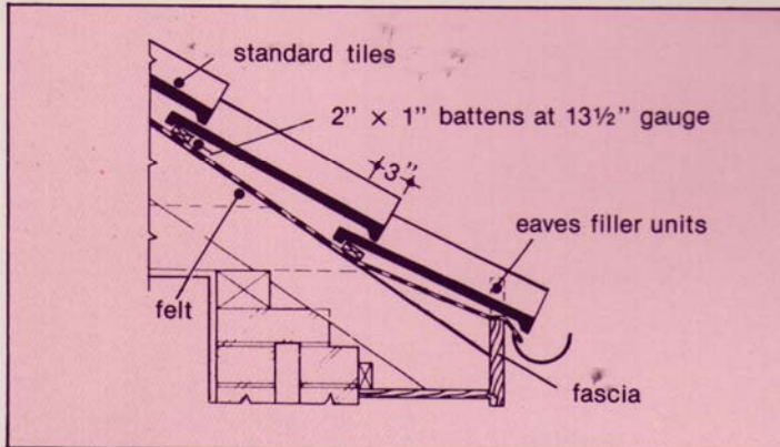
TYPICAL DETAIL AT EAVES
