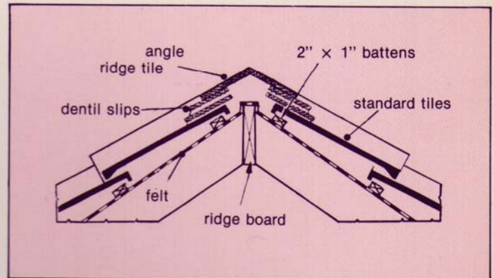
SECTION THROUGH RIDGE
