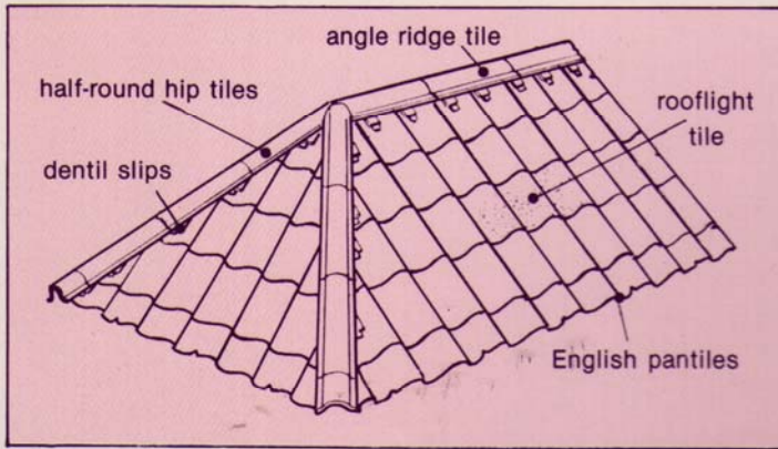
PERSPECTIVE SKETCH SHOWING TYPICAL DETAILS OF ROOF
